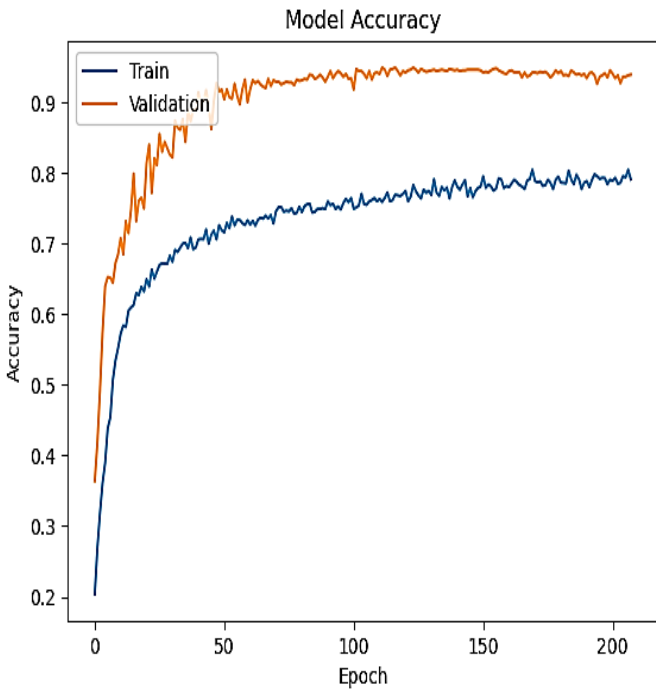
Fig. 5. Accuracy graph of the model
